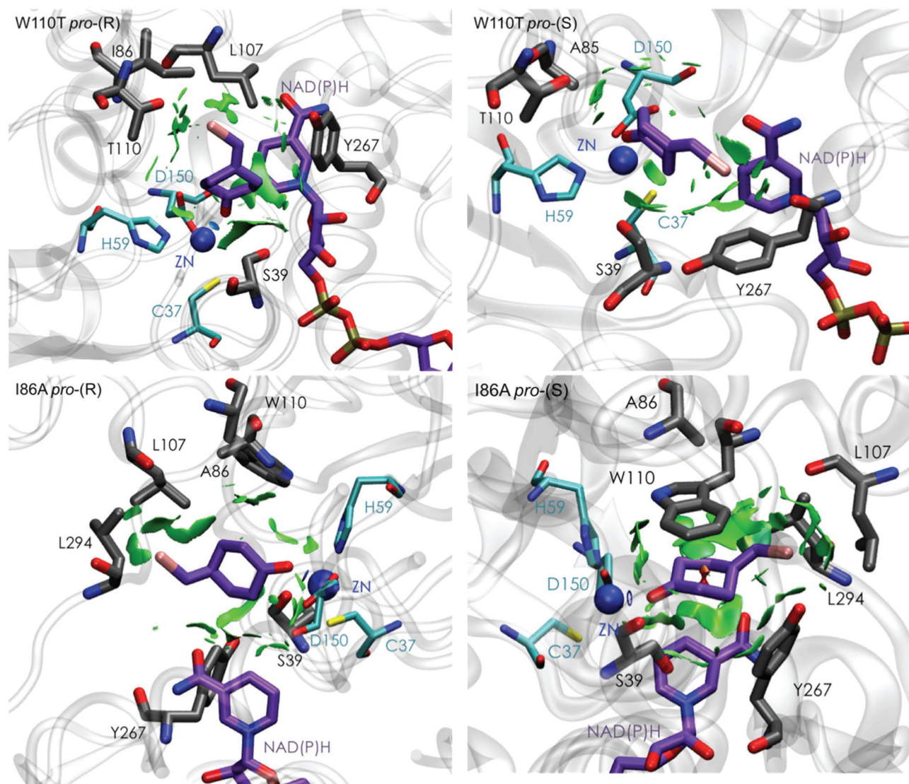
Fig. 5 Representation of the non-covalent interactions for pro-S and pro-R conformations of 1a in the active site pocket of TbSADH W110T (top) and TbSADH I86A (down) enzymes, computed with the computational tool NCIPLOT. 34,35
