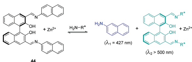
Fig. 23 Structure and proposed mechanism of 44 for detection of chiral functional amines.
