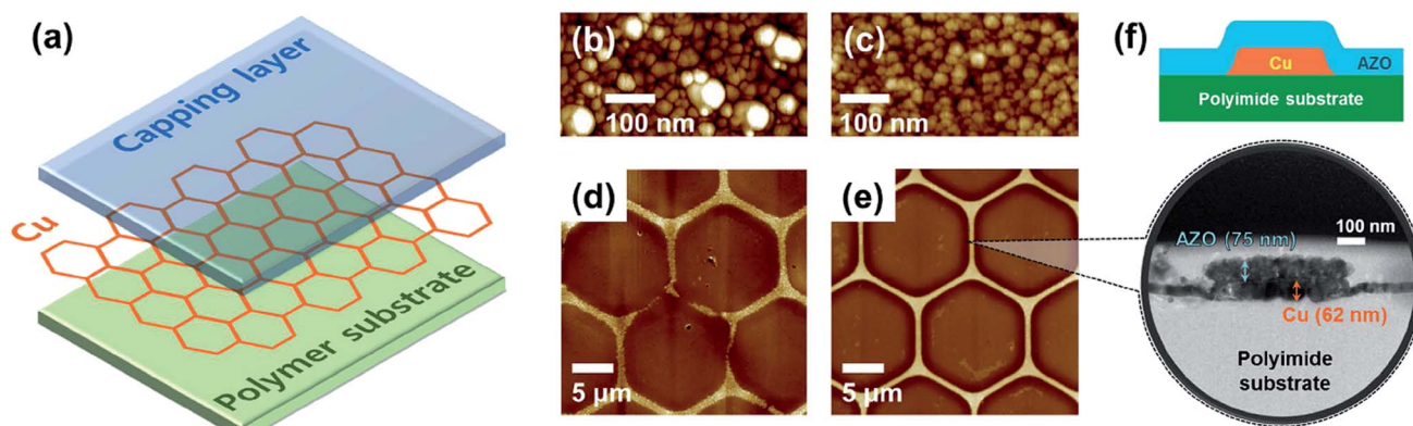
Fig. 4 (a) Structure of the Cu mesh hybrid electrode. (b) and (c) AFM topography images of Cu thin films on polyimide substrates fabricated using a polycrystalline Cu target and a single-crystal Cu target, respectively. (d) and (e) AFM topography images of Cu mesh electrodes fabricated by wet etching using the two types of Cu thin films in (b) and (c), respectively. (f) Illustration and HRTEM image of the cross-sectional structure of a Cu mesh hybrid electrode with Al:ZnO as the capping layer and polyimide as the polymer substrate (reproduced with permission. Copyright 2015, American Chemical Society). 73
