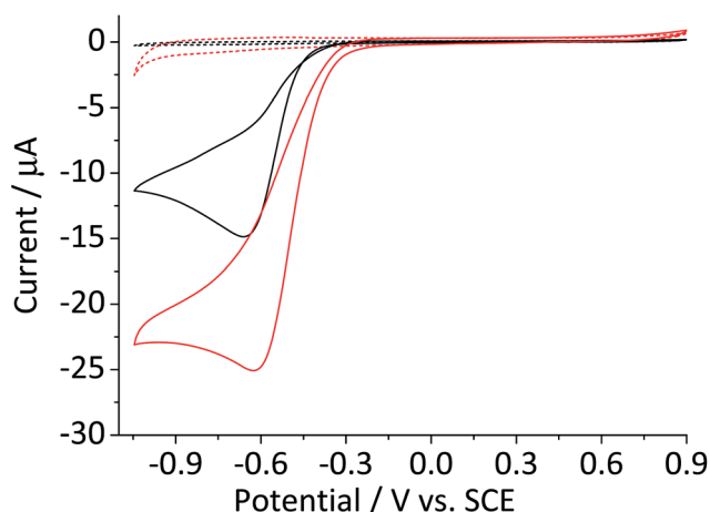
Fig. 1 Cyclic voltammograms of the oxygen reduction reaction at a bare glassy carbon electrode (black) and that modified with 2.4 \times 10^{-5} \text{ g cm}^{-2} of hematite nanoparticles (red) collected in \text{O}_2 saturated 20 mM KCl at the scan rate of 0.01 \text{ V s}^{-1} . The results of the two electrodes in the \text{O}_2 -free condition are also indicated with dashed lines of the same color. Potential is reported against a Standard Calomel Electrode (saturated KCl, SCE) throughout this article.
