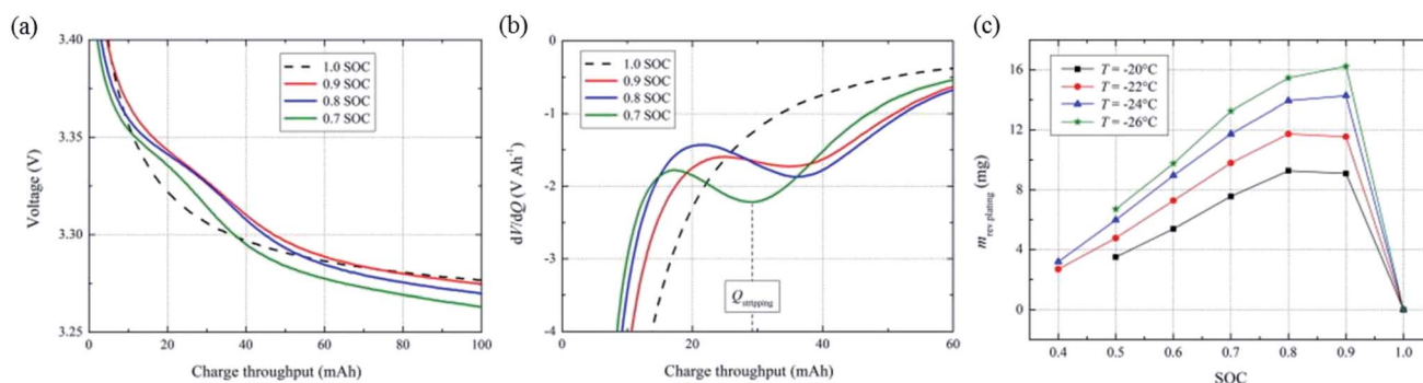
Fig. 2 (a) Discharge voltage profiles and (b) differential voltage plots ( dV/dQ ) of the 26650-type \text{LiFePO}_4/\text{graphite} battery after 1 C charging to different SOC levels at -20^\circ\text{C} , and (c) reversible lithium calculated from the dV/dQ plots (adapted from ref. 10).
