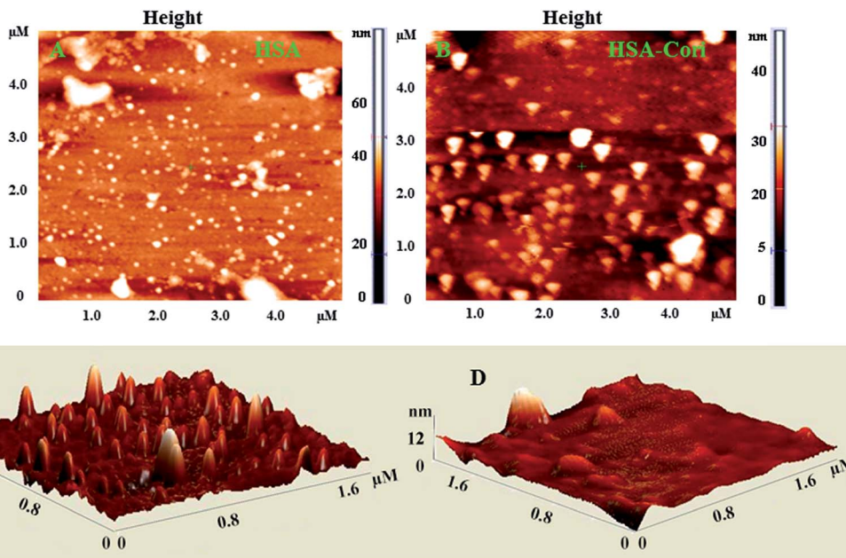
Fig. 5 2D AFM images of (A) free HSA (B) HSA–corilagin complex. The corresponding 3D images are given by (C) and (D) respectively, scan areas are given in brackets.
