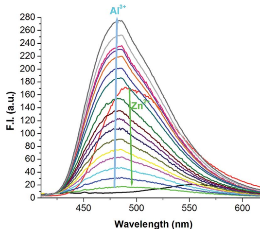
Fig. 5 Selectivity for Al 3+ over the H 2 SAL-NH–Zn 2+ complex.
