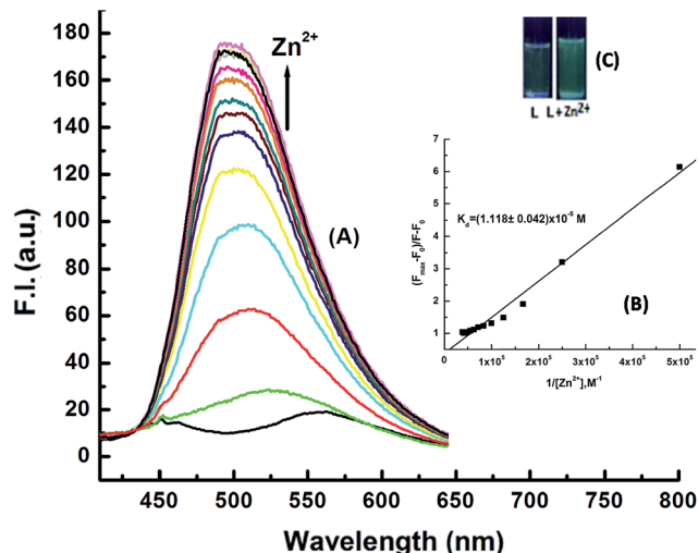
Fig. 4 (A) Fluorescence titration of H 3 SAL-NH (20 μM) in HEPES buffer at pH 7.2 recorded in THF : H 2 O (6 : 4, v/v) with the gradual addition Zn(NO 3 ) 2 ·6H 2 O with λ ex = 398 nm and λ em = 498 nm. (B) B–H plot of F.I. vs. 1/[Zn 2+ ]; (C) UV-exposed emission image of H 3 SAL-NH with Zn 2+ .
