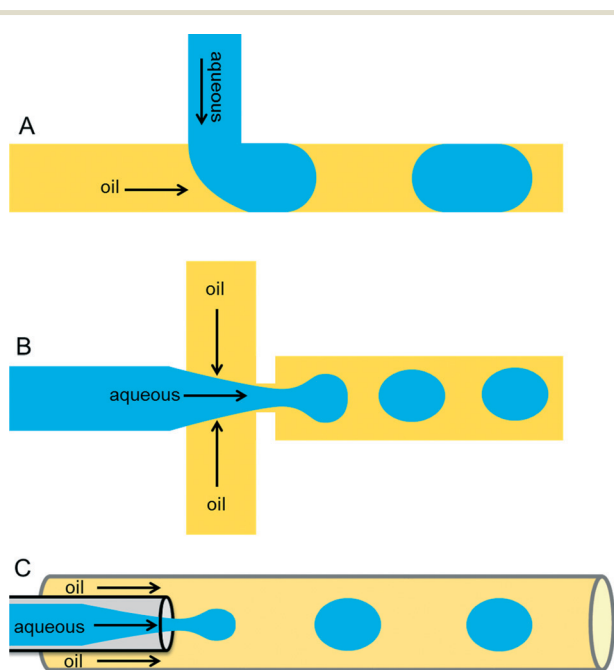
Fig. 1 Different microfluidic drop maker geometries. (A) In the T-junction geometry, the perpendicular flow of the aqueous phase is sheared by oil and thereby generates droplets. (B) The flow-focusing geometry produces droplets by shearing the aqueous stream from two directions. (C) In the co-flow geometry, the aqueous phase is forced through a capillary, which is placed co-axially inside a bigger capillary, through which immiscible oil is pumped.
