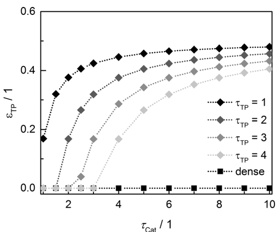
Fig. 9 Transport pore fraction for the optimized cases compared to the non-optimized, dense case as a function of catalyst tortuosity and transport pore tortuosity.
