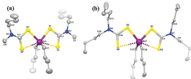
Fig. 10 Molecular structures of (a) [\text{Sn}(\text{C}_4\text{H}_9)_2(\text{S}_2\text{CNMe}^n\text{Bu})_2] and (b) [\text{Sn}(\text{C}_4\text{H}_9)_2(\text{S}_2\text{CN}^n\text{Bu})_2] with 50% ellipsoidal probability level. All the H atoms on carbon frames are removed for clarity. Reproduced with permission from ref. 97. Copyright 2014 American Chemical Society.
