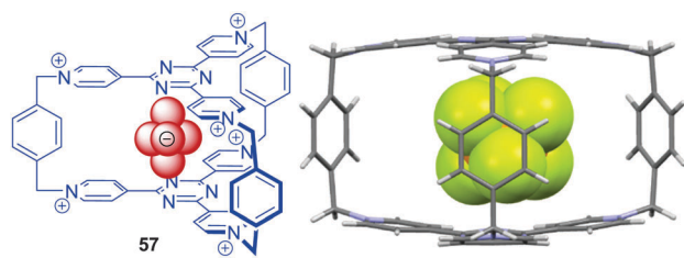
Fig. 31 Molecular structure and solid state structure of the Blue-Cage 6+ encapsulating an PF_6^- anion as reported by Stoddart and co-workers (disordered anions and solvent molecules omitted for clarity). 65
