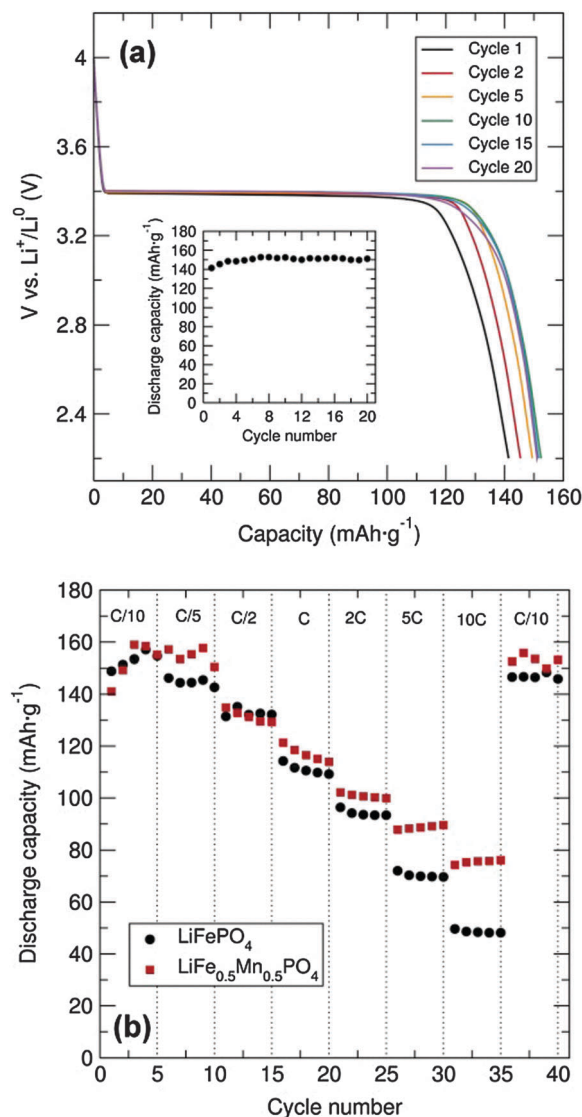
Fig. 4 (a) Cycling performance and capacity fading (inset) of C/ \text{LiFePO}_4 prepared from [\text{Fe}(\text{O}^i\text{Bu})_2(\text{THF})]_2 alkoxide precursor (mixed with C black and PTFE in 60 : 30 : 10 weight%) between 2.2 and 4.0 V at C/20 rate. (b) Rate performance of C/ \text{LiFePO}_4 and C/ \text{LiFe}_{0.5}\text{Mn}_{0.5}\text{PO}_4 (mixed with C black and PTFE in 60 : 30 : 10) at different charge-discharge C rates.
