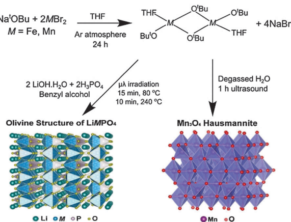
Fig. 1 Reaction schematic for the synthesis of \text{LiMPO}_4 ( M = \text{Fe} or \text{Mn} ) and \text{Mn}_3\text{O}_4 using metal alkoxide precursors.
