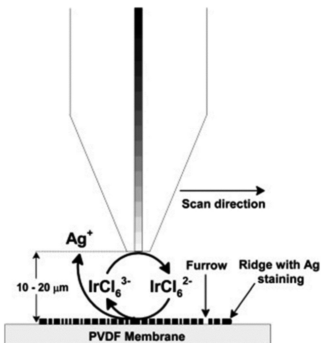
Fig. 13 Schematic (not to scale) of the operating principle for SECM imaging of silver stained fingerprints on the PVDF membrane using \text{IrCl}_6^{3-} oxidation ( E_{\text{tip}} = 0.8 V vs. Ag QRE) at the tip. 99 Reproduced from ref. 99 with permission from the Elsevier.
