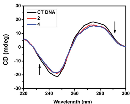
Fig. 9 CD spectra of CT DNA (200 µM) in the absence and presence of 40 µM of complex 2 and 4.
