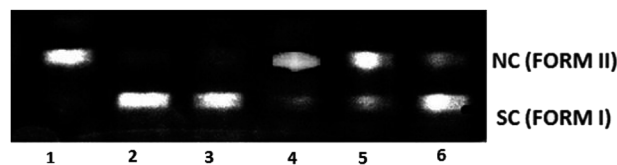
Fig. 10 Cleavage of supercoiled pUC19 DNA (40 µM) by complexes 1–5 in a buffer containing 5% DMF/5 mM Tris–HCl/50 mM NaCl at pH = 7.2 and 37 °C with an incubation time of 3 h. Lane 1, DNA control; lane 2, DNA + 1 (150 µM); lane 3, DNA + 2 (150 µM); lane 4, DNA + 3 (150 µM); lane 5, DNA + 4 (150 µM); lane 6, DNA + 5 (150 µM). Forms SC and NC are supercoiled and nicked circular DNA, respectively.
