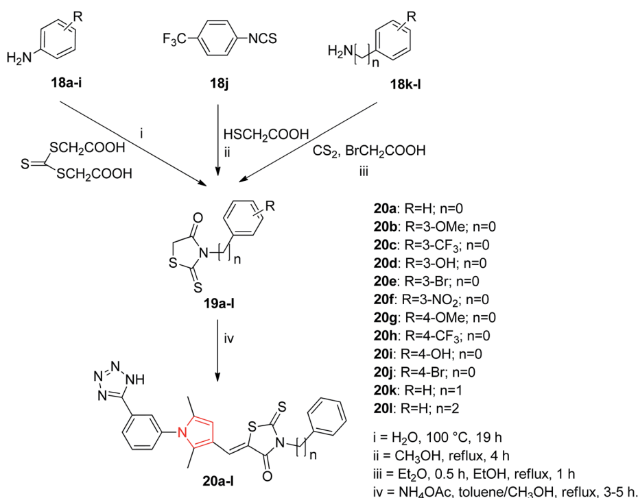
Scheme 2 Synthesis of rhodanine derivatives.
