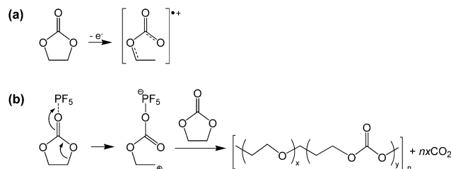
Fig. 11 Possible mechanism for the EC decomposition via strong Lewis acid, PF 5 . Reproduced with permission. 68
