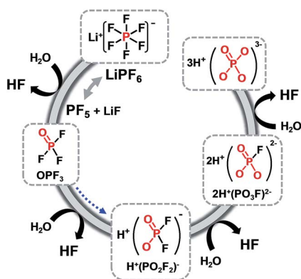
Fig. 18 Hydrolysis reactions of \text{LiPF}_6 salt in the presence of trace water in the cell.
