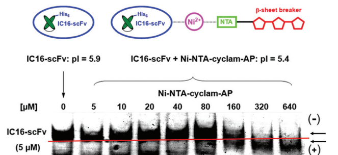
Fig. 7 Native PAGE for verification of complex formation between IC16-scFv (5 \mu M) and increasing amounts of Ni-NTA-cyclam-AP. Gel pH = 6.7.
