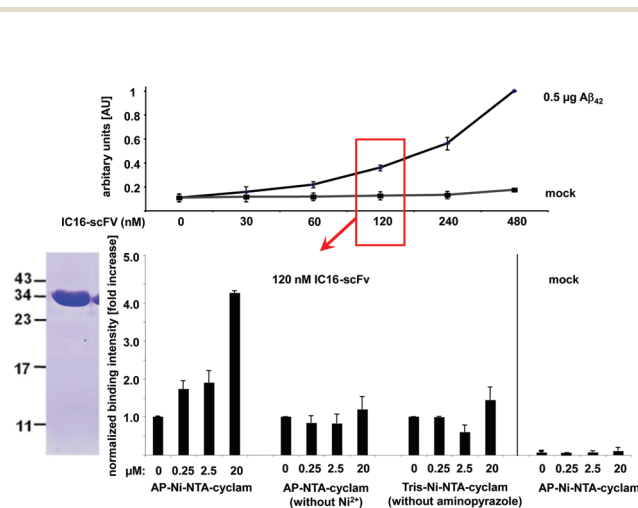
Fig. 8 ELISA-experiment for the investigation of binding properties of the self-assembled complex between AP-Ni-NTA-cyclam and IC16-scFv. Top: dose response chart of IC16-scFv binding to A \beta (1-42). Bottom: 120 nM IC16-scFv was complexed with increasing amounts of either AP-Ni-NTA-cyclam, AP-NTA-cyclam or Tris-Ni-NTA-cyclam. Binding intensities are shown in comparison to 120 nM IC16-scFv alone (n-fold increase).
