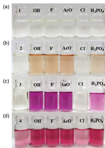
Fig. 1 Colour changes observed for 2.7 \times 10^{-5} M 1–4 in 9:1 DMSO– \text{H}_2\text{O} on addition of up to 4 equivalents of \text{OH}^- , \text{F}^- , \text{AcO}^- , \text{Cl}^- and \text{H}_2\text{PO}_4^- as sodium salts.
