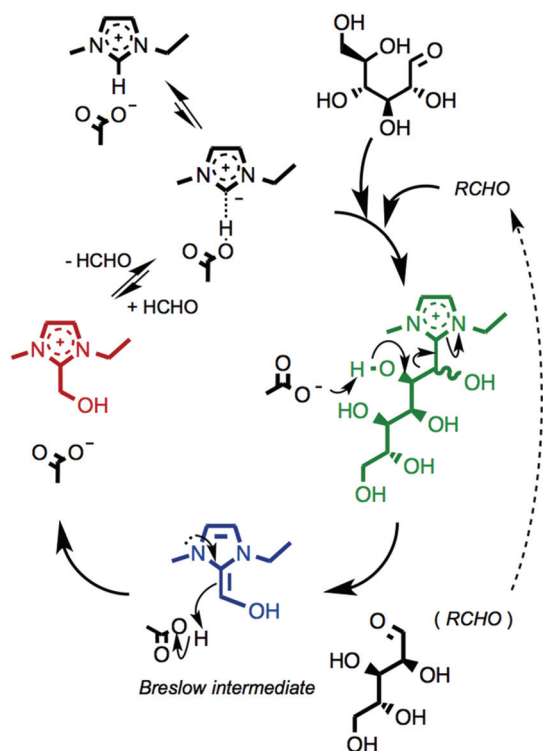
Fig. 8 Proposed scheme for condensation of [C_2C_1im][OAc] , 1a , with open-chain D-(+)-glucose, 12 , yielding the C1 adduct [C_2C_1(HO)C_1^2im]^+ , 17 (red), via a Breslow intermediate (blue). The cleaved C(n-1) aldehyde fragment can react again with the parent ionic liquid, accounting for the intermediate adducts C5, C4, C3 and C2.
