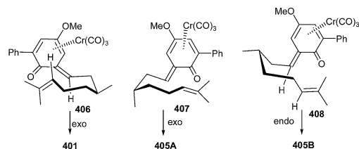
Scheme 88 Diastereoselective synthesis of hexahydrobenzopyrans via a chair transition state of a Cr complexed o -QM.
