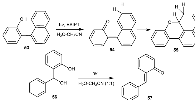
Scheme 13 Generation of o -QM by ESIPT.
