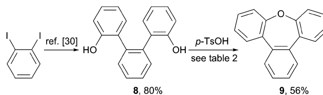
Scheme 3 Synthesis of tribenz[b,d,f]oxepin 9 .
