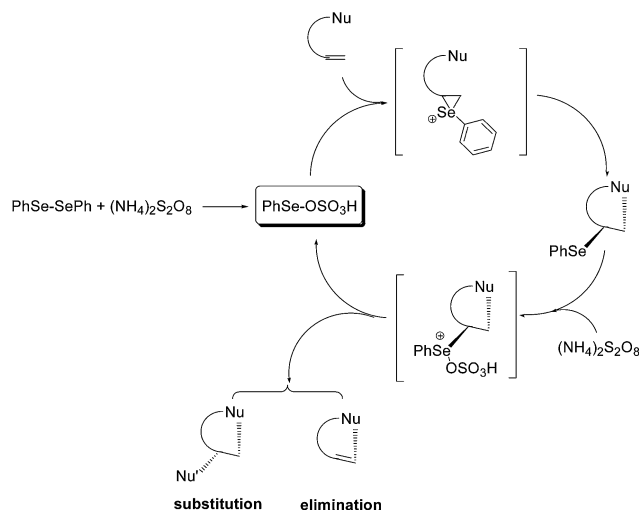
Scheme 23 One pot selenenylation–deselenenylation for the synthesis of heterocycles.
