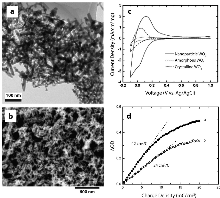
Fig. 3 WO 3 nanocrystals for electrochromic devices. (a) TEM micrograph of WO 3 nanocrystals synthesized by HWCVD. (b) SEM micrograph of WO 3 nanocrystal electrochromic electrode. (c) Cyclic voltammograms (scan rate: 20 mV s -1 ) displaying the enhanced charge capacity of nanocrystalline WO 3 . (d) Change in optical density at 670 nm upon charging a mixture of nanorods and nanospheroids (open circles) and nanospheroids only (closed circles). Reprinted with permission from ref. 22. Copyright © 2006 WILEY-VCH Verlag GmbH & Co. KGaA, Weinheim.
