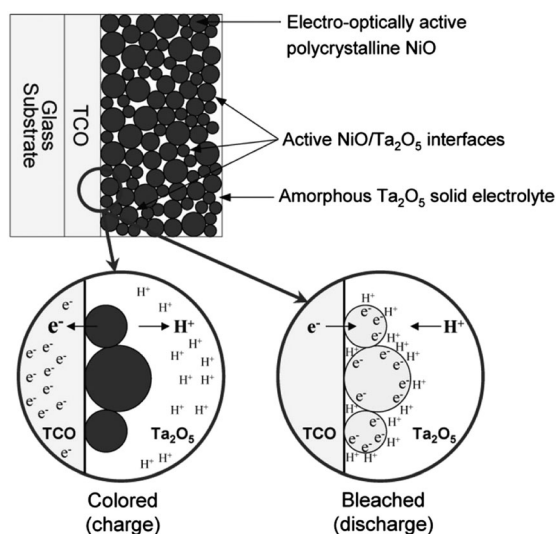
Fig. 4 Nanostructured NiO electrochromic device. NiO nanoparticles are dispersed in an amorphous Ta 2 O 5 matrix, which also acts as an electrolyte for protons. When electrons are injected, protons in the electrolyte adsorb onto the particle surfaces and the nickel ions are reduced at the surface through a pseudocapacitive process. As a result, the electrode bleaches according to the anodic colouration mechanism of NiO. Reprinted with permission from ref. 23. Copyright 2005 The Electrochemical Society.
