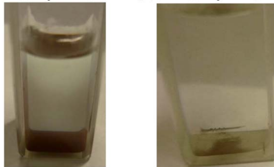
Fig. 1 Visual observation of the disproportionation of \text{CuBr} in DMSO with 0.5 equivalent (a) and 1 equivalent (b) of \text{Me}_6\text{-TREN} after 3 h at 25 °C. Conditions: DMSO = 1.8 mL; (a) [\text{CuBr}]/[\text{Me}_6\text{-TREN}] = 1/0.5 and (b) [\text{CuBr}]/[\text{Me}_6\text{-TREN}] = 1/1 .
