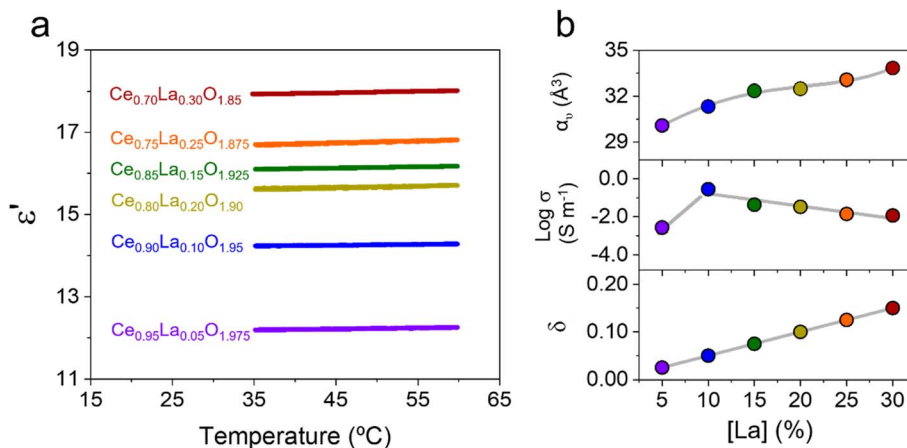
Fig. 3 Lanthanum doping enhances dielectric polarization through ionic and defect mechanisms. (a) Relative dielectric constant (ε') as a function of temperature for La-doped samples; (b) polarizability (α v ), DC conductivity, and intrinsic V O 2- content (δ Ext ) versus La content, showing the decoupling between transport and dielectric response at high doping levels.
