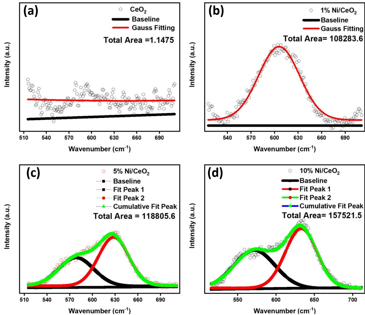
Fig.2 Deconvolution of Raman Spectra for (a) CeO 2 and (b), (c), & (d) for 1%, 5%, 10% Ni/CeO 2 , respectively.
