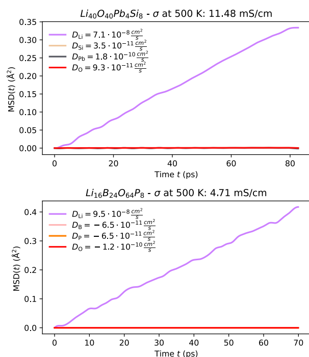
Fig. 10 MSD plot of Li along with host-lattice species of \text{Li}_{10}\text{Si}_2\text{PbO}_{10} and \text{Li}_2\text{B}_3\text{PO}_8 at 500 K from FPMD.
