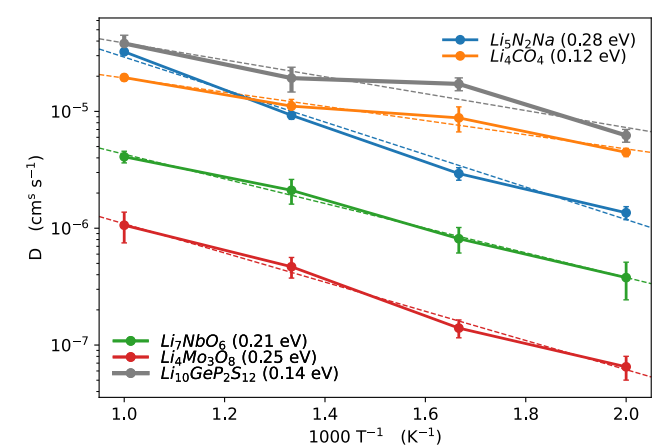
Fig. 11 Diffusion coefficients derived from our FPMD simulations for the most promising oxides and nitrides. The dashed line represents the best-fit line, with the slope corresponding to the activation barriers, indicated in brackets (eV). We additionally show LGPS for comparison, with data taken from the work of Kahle et al. 117 .
