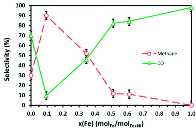
Fig. 11 Effect of Fe content on CH 4 and CO selectivity in comparison to sole metals (this figure has been reproduced from ref. 82 with permission from RSC, copyright 2018).
