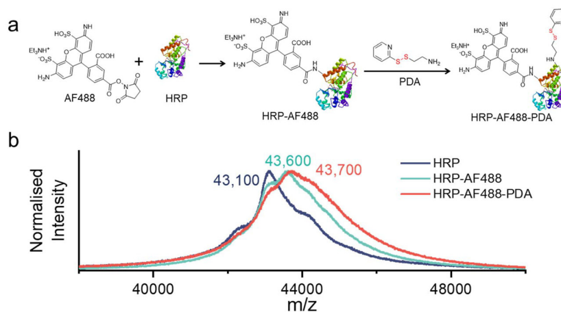
Fig. 3 (a) Reaction scheme of the modification of HRP with the fluorescent dye AF488 and disulphide bonds (PDA). (b) MALDI-TOF MS spectra in the [M + X]^+ ( X: \text{Na} or \text{H} ) range of HRP, HRP-AF488, and HRP-AF488-PDA.
