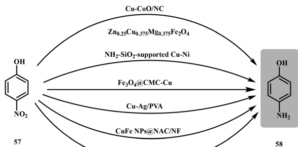
Scheme 28 Various copper-catalysts used in reduction reaction.
