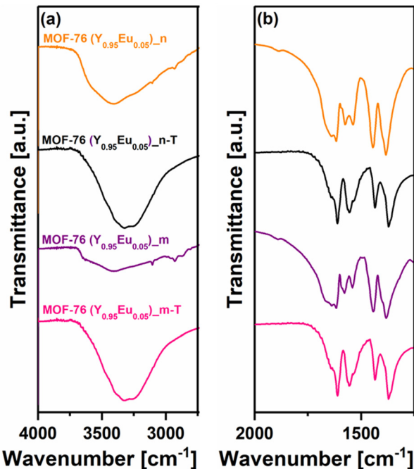
Fig. 9 FTIR spectra of the synthesized MOF-76( Y_{0.95}Eu_{0.05} ) n (orange) compound and after sonication for 15 min in H 2 O (MOF-76( Y_{0.95}Eu_{0.05} ) n-T , black), MOF-76( Y_{0.95}Eu_{0.05} ) m (purple) material and after sonication treatment for 60 min in H 2 O (MOF-76( Y_{0.95}Eu_{0.05} ) m-T , pink), (a) from 4000–2900 cm -1 and (b) from 2000–1250 cm -1 .
