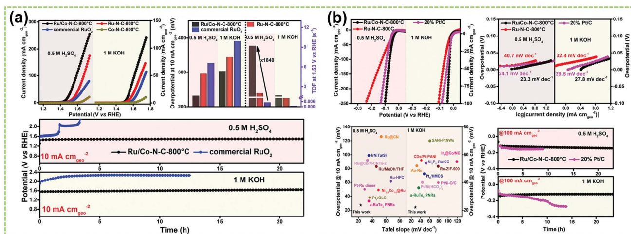
Fig. 22 The overall water electrolysis performance of DACs in wide-pH conditions. (a) Electrochemical OER performance of Ru/Co-N-C-800 °C compared with other samples. Above left: OER polarization curves were obtained at a scan rate of 5 mV s -1 in N 2 -saturated 0.5 M H 2 SO 4 and 1 M KOH. Above right: comparison of overpotential to achieve a current density of 10 mA cm -2 and TOF value at 1.53 V versus RHE in 0.5 M H 2 SO 4 and 1 M KOH. Below: the chronopotentiometry of Ru/Co-N-C-800 °C and commercial RuO 2 in 0.5 M H 2 SO 4 and 1 M KOH. (b) Electrochemical HER performance of Ru/Co-N-C-800 °C compared with other samples. Above left: HER polarization curves obtained at a scan rate of 5 mV s -1 in N 2 -saturated 0.5 M H 2 SO 4 and 1 M KOH. Above right: the corresponding Tafel plots in 0.5 M H 2 SO 4 and 1 M KOH. Below left: comparison of overpotential at 10 mA cm -2 and Tafel slope with previously reported HER catalysts in acid and alkaline conditions. Below right: the chronopotentiometry curves of Ru/Co-N-C-800 °C and commercial Pt/C in 0.5 M H 2 SO 4 and 1 M KOH 169 (reproduced with permission from ref. 169 copyright 2022, John Wiley and Sons).
