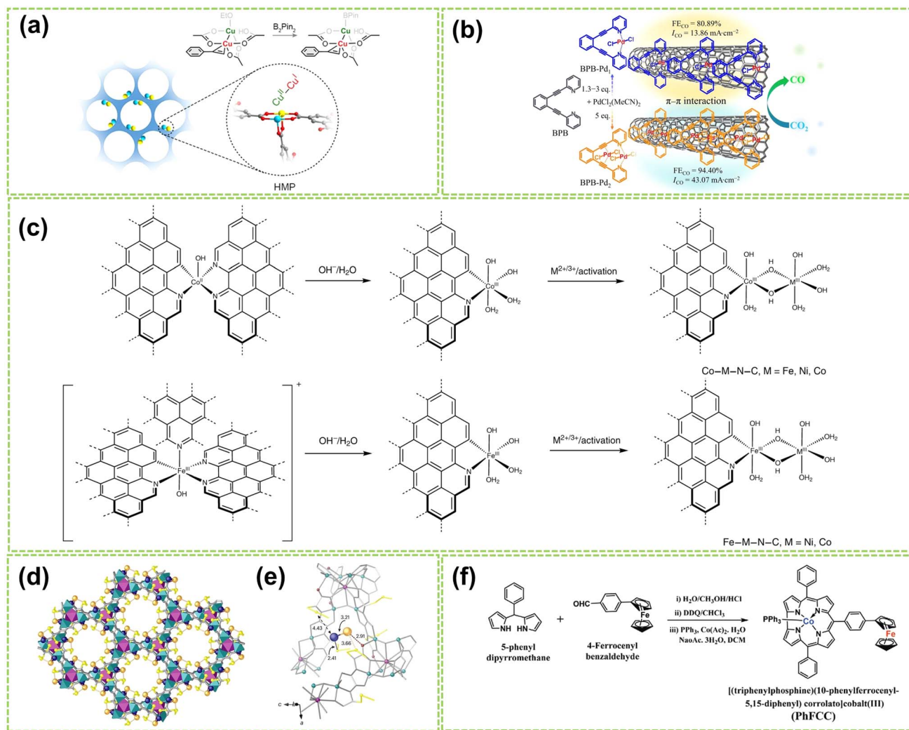
Fig. 9 Structure illustration of molecular DACs. (a) Schematic diagram and structural formula of the heterovalent metal pair (HMP) site of copper. The color scheme for the atom: cyan for \text{Cu}^{\text{II}} , yellow for \text{Cu}^{\text{I}} , red for O, and gray for \text{C}^{76} (reproduced with permission from ref. 76 copyright 2024, ACS). (b) The preparation strategy for BPB- \text{Pd}_1 and BPB- \text{Pd}_2 and the electrocatalytic \text{CO}_2 reduction performance of catalysts supported on carbon nanotubes 77 (reproduced with permission from ref. 77 copyright 2024, Springer Nature). (c) A scheme showing the formation of DACs from the Co-based and Fe-based single-atom precatalysts. The dashed bonds connected to aromatic rings indicate extended N-doped carbon layers 78 (reproduced with permission from ref. 78 copyright 2021, Springer Nature). (d) Formation of \text{Pd}_1 - \text{Au}_1 dimers showing the structures of \text{Pd}_1\text{Au}_2@1 determined by SCXRD. Copper and strontium atoms from the network are represented by cyan and purple polyhedra. Organic ligands are depicted as grey sticks and thioether groups as yellow sticks in all cases. Orange and blue spheres represent gold and palladium atoms, respectively, in \text{Pd}_1 - \text{Au}_1 dimers. Blue, orange, and red dotted lines represent the \text{Pd}\cdots\text{S} , \text{Au}\cdots\text{S} , and \text{Au}\cdots\text{O} interactions. (e) Details of X-ray crystal structure showing the main host-guest interactions and related structural parameters of \text{Pd}_1 - \text{Au}_1 dimers 79 (reproduced with permission from ref. 79 copyright 2024, Springer Nature). (f) Synthetic route for PhFCC 80 (reproduced with permission from ref. 80 copyright 2021, John Wiley and Sons).
