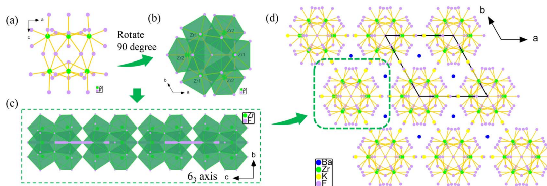
Fig. 1 (a and b) cis-[Zr_6F_{34}]^{10-} cluster at the ac and ab plane; (c) the \{[Zr_6F_{34}]^{7-}\}_\infty chain along the c -axis; (d) the aligned arrangement of the \{[Zr_6F_{34}]^{7-}\}_\infty anionic chains and whole structure of K_3Ba_2Zr_6F_{31} viewed along the c -axis.
