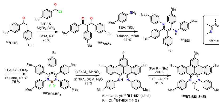
Scheme 1 Synthetic route towards {}^{\text{tBu}}\text{BT-BDI} and its \text{ZnEt} complex.
