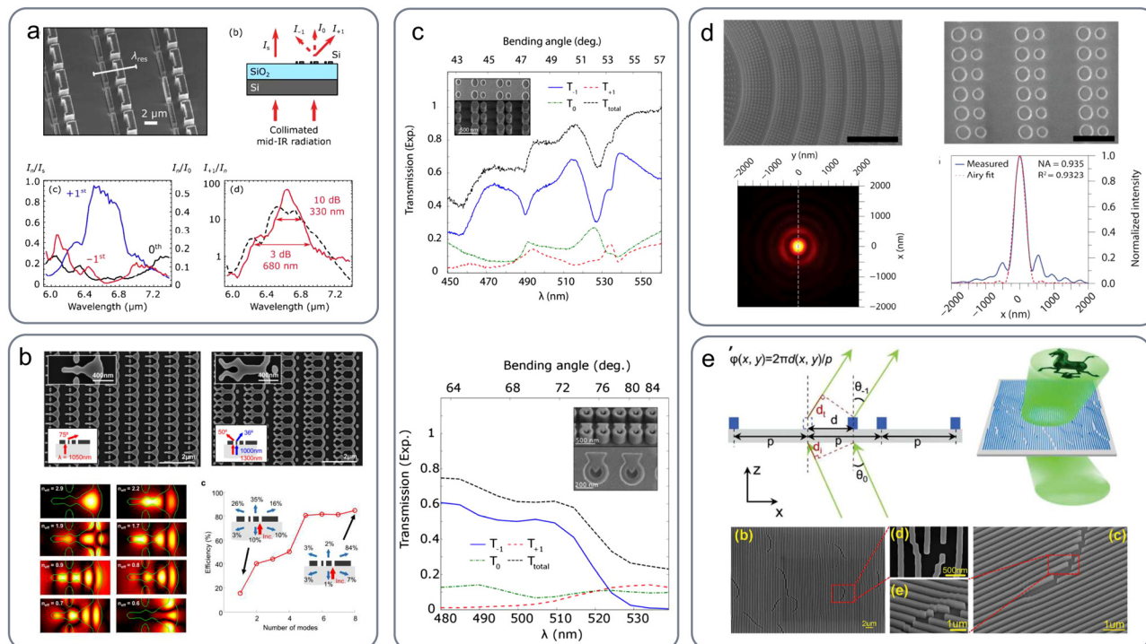
Fig. 5 Dielectric implementations of metagratings. (a) Silicon-based metagrating for high-angle light bending at mid-infrared frequencies ( 6.5\ \mu\text{m} ). 140 A two-part bianisotropic metamolecule supporting four resonances is proposed to selectively promote only one of the available radiation channels. Adapted with permission from ref. 140. Copyright 2018, American Chemical Society. (b) Silicon-based metagrating for light bending and beam splitting at near-infrared frequencies. 141 A freeform geometry has been proposed based on inverse design and adjoint optimization. Adapted with permission from ref. 141. Copyright 2017, American Chemical Society. (c) Titanium dioxide metagrating for high-angle light bending at visible wavelengths ( \sim 500\ \text{nm} ). 142 Adapted with permission from ref. 142. Copyright 2017, American Chemical Society. (d) Spatially-modulated metagrating for a metalens with near-unity numerical aperture, enabled by the ability to efficiently bend light at high angles. 143 The material is amorphous silicon and the operation wavelength is 715\ \text{nm} . Adapted with permission from ref. 143. Copyright 2018, American Chemical Society. (e) \text{SiN}_x -based metagrating with a spatially-modulated period for arbitrary wavefront manipulation in the visible region. 144 Adapted with permission from ref. 144. Copyright 2020, Royal Society of Chemistry.
