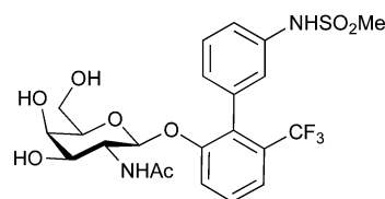
107 \text{IC}_{50} = 34 \text{ nM}
