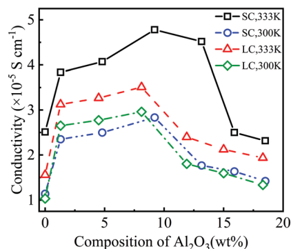
Fig. 4 Conductivities of SPE with different mass fractions of Al 2 O 3 .
