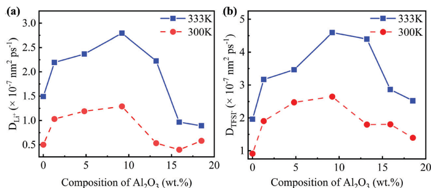
Fig. 3 Diffusivities of (a) Li + and (b) TFSI - at different temperatures in the SC system.
