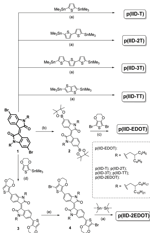
Scheme 2 Synthesis of isoindigo-polymers p(IID-T) , p(IID-2T) , p(IID-3T) , p(IID-TT) , p(IID-EDOT) and p(IID-2EDOT) . Reagents and conditions: (a) \text{Pd(PPh}_3)_4 , toluene, 100^\circ\text{C} for 24 h; (b) \text{B}_2(\text{Pin})_2 , KOAc, Pd(dppf) \text{Cl}_2 \cdot \text{DCM} , 1,4-dioxane, 80^\circ\text{C} for 18 h; (c) \text{Pd(PPh}_3)_4 , \text{K}_2\text{CO}_3 in \text{H}_2\text{O} , toluene, 85^\circ\text{C} for 72 h; (d) \text{Pd(PPh}_3)_4 , toluene, 90^\circ\text{C} for 16 h; (e) NBS, THF, 0^\circ\text{C} to r.t. for 24 h.
