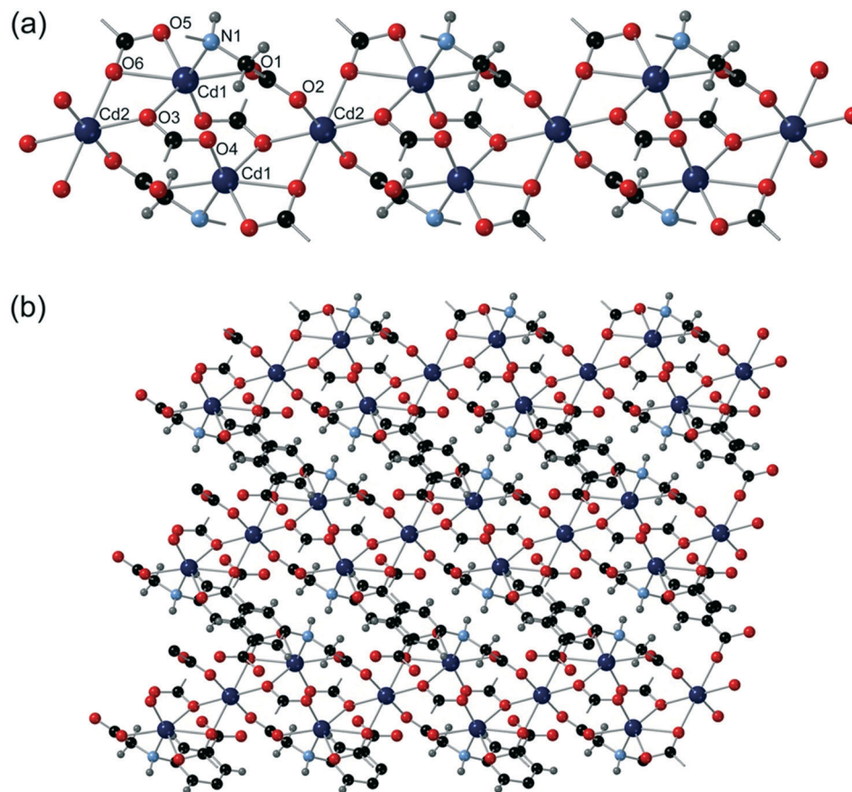
Fig. 4 The structure of compound 4 showing (a) the one-dimensional chains with the bulk of the cmal ligands removed for clarity and (b) the dense three-dimensional network adopted.
