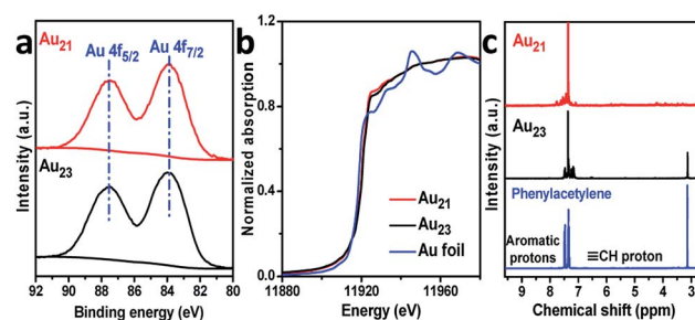
Fig. 5 (a) Au 4f XPS and (b) Au L 3 -edge XANES profiles of \text{Au}_{21}(\text{SR})_{12}(\text{Ph}_2\text{PCH}_2\text{PPh}_2)_2 and \text{Au}_{23}(\text{SR})_{16} . (c) The 1 H NMR spectra of Au-acetylide species.
