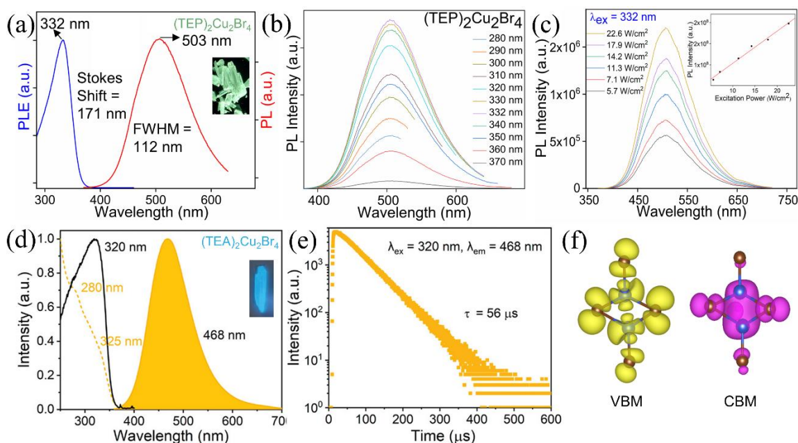
Fig. 9 PL and PLE spectra of (a) (\text{TEP})_2\text{Cu}_2\text{Br}_4 and (d) (\text{TEA})_2\text{Cu}_2\text{Br}_4 at room temperature. Insets show the single crystals of the corresponding compounds under UV irradiation. (b) Excitation-dependent PL spectra of (\text{TEP})_2\text{Cu}_2\text{Br}_4 . (c) Power-dependent PL spectra of (\text{TEP})_2\text{Cu}_2\text{Br}_4 . Inset shows the corresponding plot of the excitation power vs PL intensity. Reproduced from ref 62. Copyright 2024 John Wiley and Sons. (e) Time-resolved PL spectrum of (\text{TEA})_2\text{Cu}_2\text{Br}_4 crystals at room temperature. Reproduced with permission from ref 75. Copyright 2022 John Wiley and Sons. (f) Partial charge density contours of the hole (yellow) and electron (purple) in the exciton of
