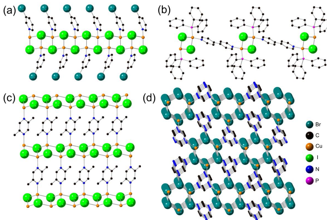
Fig. 7 Structures of select L_m\text{Cu}_n\text{X}_n compounds: (a) 1\text{D-CuI}(3\text{-Br-py}) , 157 (b) 1\text{D-Cu}_2\text{I}_2(\text{tpb})_2(4,4'\text{-bpy}) , 173 (c) 2\text{D-CuI}(2,5\text{-dm-pz})_{0.5} , 175 (d) 3\text{D-CuI}(\text{tz})_{0.5} . 158 Inset shows the atomic legends. Orange, green, olive, blue, pink and black spheres represent copper, iodide, bromide, nitrogen, phosphorous and carbon, respectively. Hydrogens are omitted for clarity.
