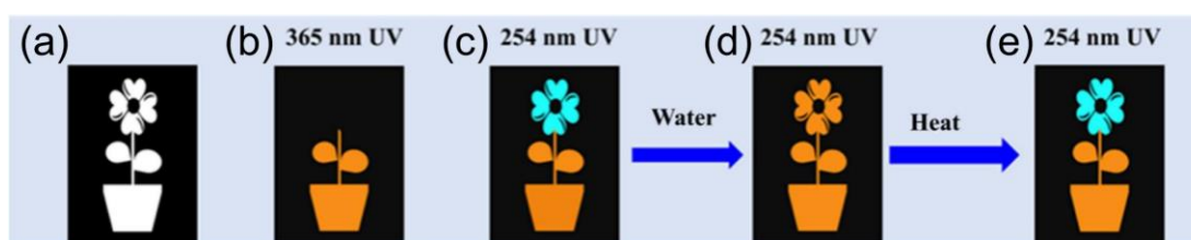
Fig. 23 Demonstration of triple-mode anti-counterfeiting application using interconvertible (\text{TPA})\text{CuBr}_2 (cyan) and (\text{TPA})_2\text{Cu}_4\text{Br}_6 (orange). The pattern of flowerpot and petals under (a) daylight, (b) 365 nm UV light, (c) 254 nm UV light. (d) Whole pattern appears orange after water treatment, under 254 nm UV light. (e) The cyan emission of (\text{TPA})\text{CuBr}_2 (flower) has been recovered after heat treatment, under 254 nm UV light. Reproduced with permission from ref 82. Copyright 2023 Elsevier.
