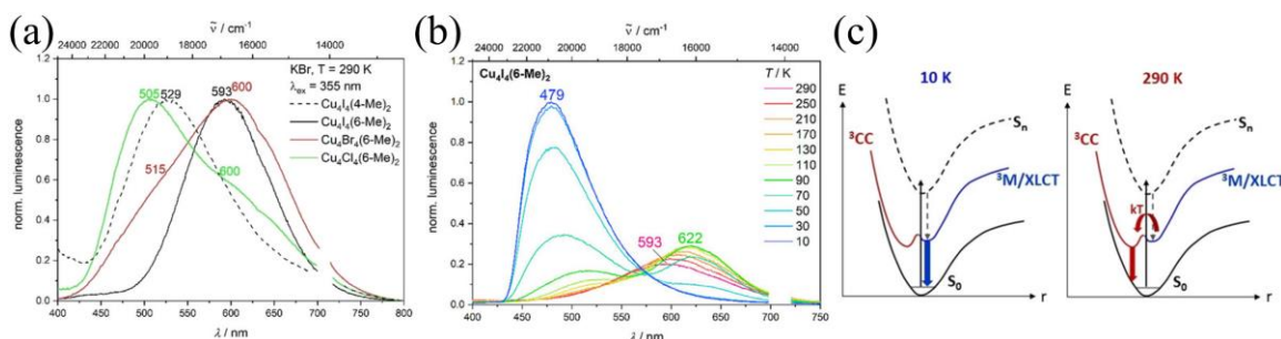
Fig. 16 (a) Photoluminescence emission spectra of Cu 4 I 4 (4-Me) 2 , Cu 4 I 4 (6-Me) 2 , Cu 4 Br 4 (6-Me) 2 , Cu 4 Cl 4 (6-Me) 2 at 290 K excited at 355 nm (where 6-Me = 2-(diphenylphosphino)pyridine). (b) Temperature dependent emission spectra of Cu 4 I 4 (6-Me) 2 recorded in the temperature range 10 K – 290 K. (c) Simplified energy diagram of the complex Cu 4 X 4 (6-Me) 2 , where blue emission associated with M/XLCT at 10 K (left) and red emission associated with CC at 290 K (right) are represented. Reproduced with permission from ref 186. Copyright 2020 John Wiley and Sons.
