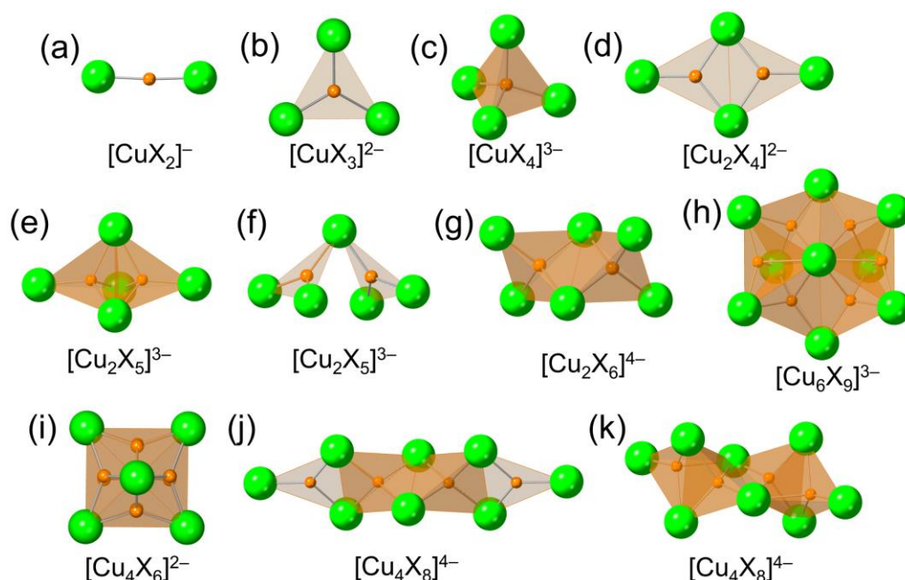
Fig. 2 Structural diversity found in hybrid Cu(I) halides showcasing 0D inorganic building blocks: (a) linear, (b) trigonal planar, (c) tetrahedra, (d) edge-sharing trigonal planar dimer, (e) face-sharing tetrahedral dimer, (f) corner-sharing trigonal planar dimer, (g) edge-sharing tetrahedral dimer, (h) face-sharing tetrahedral cluster, (i) edge-sharing trigonal planar cluster, (j) edge-sharing cluster of trigonal planar and tetrahedral units, (k) face and edge-sharing tetrahedral cluster. Orange and green spheres represent copper and halide atoms, respectively.
