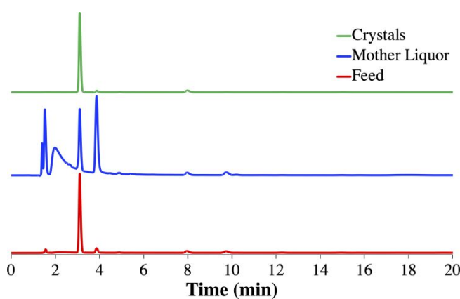
Figure 5. Normalized chromatograms for batch antisolvent crystallization experiment at room temperature (~22 °C): Red - feed of crude modafinil ( 1 ) obtained from flow synthesis protocol after 4-week storage, blue - mother
