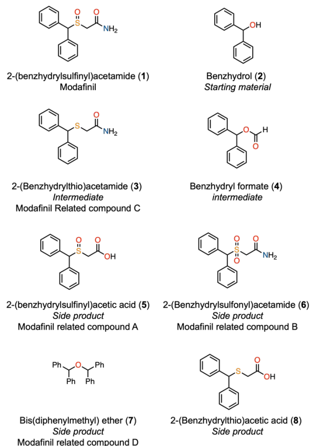
Figure 2. Structures of the main impurities related to modafinil ( 1 ). See also Table 1.
