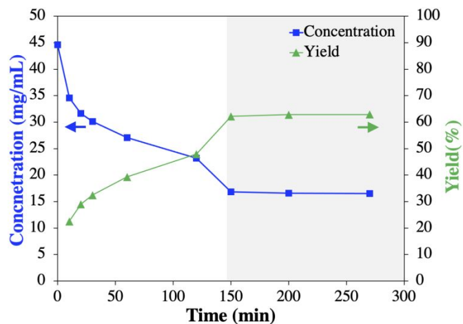
Figure 8. Results of batch cooling crystallization experiment at 5 °C: Measured modafinil ( 1 ) concentration (blue squares) and experimentally determined yield (green triangles). Grey area represents when equilibrium was reached. Arrows indicate the affiliated y-axis of the data.
