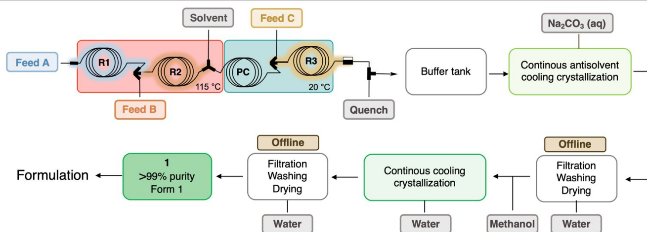
Figure 1. Top: Three-step continuous flow synthesis of modafinil ( 1 ). Bottom: Process flow diagram for synthesis and purification of 1 with all major unit operations leading to 1 in >99% purity (HPLC), including the microfluidic flow setup optimized from the literature. 38
