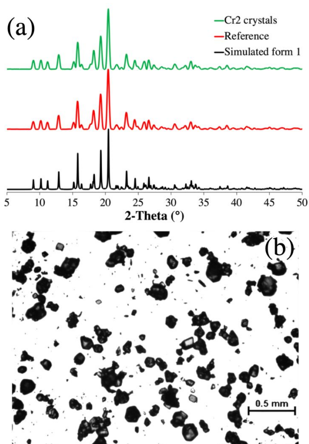
Figure 9. a. Powder X-ray diffractograms of modafinil ( 1 ). From bottom to top: simulated polymorphic form I (black, Reference Code = 236078) 59 obtained from the Cambridge Structural Database, 60 reference “as received” (red), and Cr2 crystals (green). B. Representative optical micrograph of 1 crystals obtained from Cr2.
