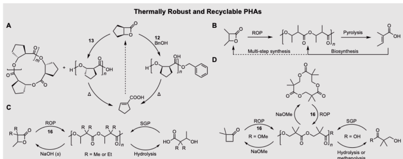
Fig. 3. Highlighted examples of thermally robust and chemically recyclable PHAs.
