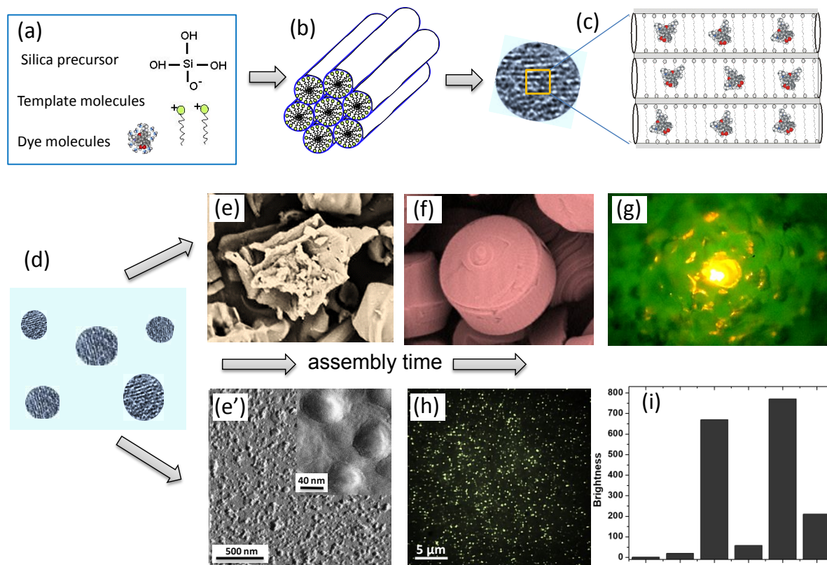
Figure 1. A schematic of the mechanism of self-assembly of ultrabright mesoporous silica particles (UMSP). (a) The building blocks of the particles: template cationic surfactant molecules, which will form liquid crystals; a mineralizable inorganic anion, deprotonated silicate; and dye molecules. (b) Deprotonated silicate condenses on the surface of the nematic liquid crystals created by the template molecules. (c) Small nematic crystals are fused into silica mesoporous structures, “seed” particles, which carry fluorescent dye molecules encapsulated inside the cylindrical channels of the particles. (d) Initially sticky and not fully polymerized seed particles of 10 – 20 nm in size will now be the building blocks for both nano and micron size UMSP. (e) The seeds assemble in larger micron-size aggregates if allowed to stay in the synthesizing bath. (f) the micron-size aggregates have further been developed into mesoporous silica shapes with well-aligned cylindrical mesochannels. (g) An example of an ultrabright fluorescent discoid illuminating the landscape of
