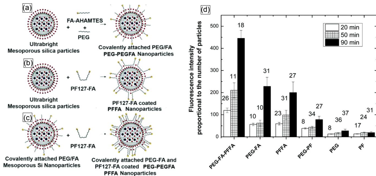
Figure 5. Schematic of the methods used to synthesize functionalized nano-UMSP. (a) Synthesis of ultrabright mesoporous silica nanoparticles with covalent attachment of folic acid and PEG. (b) Coating ultrabright mesoporous silica particles with PF127-FA. (c) Coating covalently attached PEG-FA mesoporous silica nanoparticles with PF127-FA. (d) Functional targeting of human cervical epithelial cancer (HeLa) cells using functionalized nano-UMSP. Fluorescence intensity (in arbitrary units), which is proportional to the number of nano-UMSP particles accumulated in cells after 20, 50, and 90 minutes of incubation. The number above each column bar represents the number of analyzed cells. The error bar shows one standard deviation. The results for folate functionalized nano-UMSP (SiSB-PEGFA-PFFA, SiSB-PFFA, SiSB-PEGFA) and no-folate control nanoparticles (SiSB-PEG-PF, SiSB-PEG, SiSB-PF) are shown. The experiments were repeated 3 times, with three independent wells of a multiwell plate seeded and treated in parallel, and a picture of each was acquired. [Reproduced from Ref. 71 with permission from RCS, copyright 2019.]
