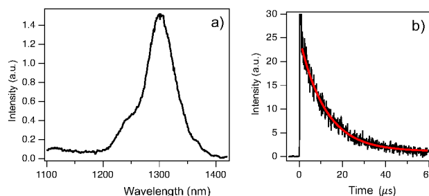
Fig. 7. Phosphorescence spectrum for Chrom7 in a \text{CD}_3\text{I} matrix at 77 K, a). The phosphorescence was recorded in the 4–19 \mu\text{s} time interval after pulsed laser excitation (532 nm, 7-ns pulse width). The phosphorescence decay (black) was measured at a 1300-nm wavelength and can be fitted to a single exponential decay (red) with a 12 \mu\text{s} lifetime, b).
