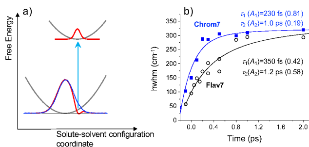
Fig. 5. Schematic diagram for the hole relaxation when excitation is into the low-energy wing of the linear absorption spectrum and excites only a narrow range of resonant sites, 84-86 a). The distribution of excited-state population may only broaden without shift, but the ground-state population bleaches to fill the hole. In b), for Chrom7 (excitation, 990 nm) and Flav7 (excitation, 1042 nm), the time evolution of the hwhm bandwidth evaluated at the short-wavelength side of the main negative \Delta A band is fitted to a two-exponential A_1 \exp(-t/\tau_1) + A_2 \exp(-t/\tau_2) function, with the fit curves and best-fit parameters shown.
