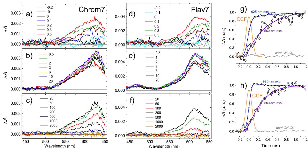
Fig. 6. Transient absorption spectra of Chrom7 (a-c) and Flav7 (d-f) in CH 2 Cl 2 at short (a, d), intermediate (b, e), and long (c, f) times following 500-nm excitation. Delay times between the excitation and probe pulses are given in the legends. Representative \Delta A kinetics traces (symbols) at the probe wavelength of 575 nm for Chrom7 in g) and 645 nm for Flav7 in h) are compared with the data (symbols) measured following 925-nm excitation within the same ESA range: 553 nm in g), and 659 nm in h). The neat CH 2 Cl 2 yields a negligibly small \Delta A signal (as shown) under the same excitation conditions. The CCF between 500-nm excitation and probe pulses is Gaussian-shaped with a 145-fs fwhm, g) and h).
