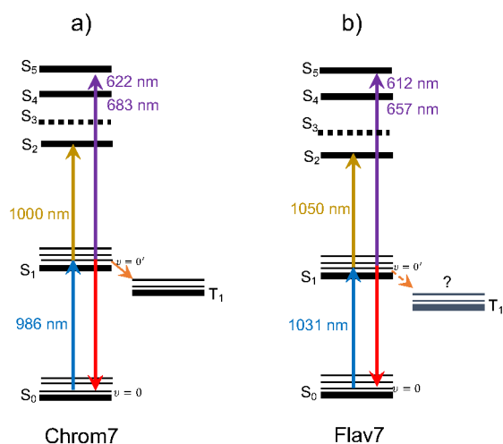
Fig. 11. Energy diagram for Chrom7, a), and Flav7, b), based on this work. The S_0 \rightarrow S_1 energy gap is 10140 and 9700 \text{cm}^{-1} based on the overlap of the 0-0' absorption and fluorescence bands at 986 and 1031 nm. The S_1 \rightarrow S_2 and S_0 \rightarrow S_1 transitions are nearly isoenergetic, and the S_n states are found to be within 100 \text{cm}^{-1} of each other at \sim 26150 \text{ cm}^{-1} . The S_3 position is only tentatively shown because near-IR ESA attributed to the S_1 \rightarrow S_3 transition is weak and diffuse. The T_1 state is at 7750 \text{cm}^{-1} above S_0 for Chrom7 and is assumed, see the text, at 7140 \text{cm}^{-1} or lower for Flav7.
