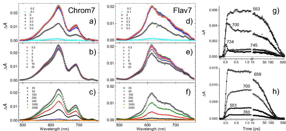
Fig. 4. Transient absorption spectra of Chrom7 (a-c) and Flav7 (d-f) in \text{CH}_2\text{Cl}_2 at short (a, d), intermediate (b, e), and long (c, f) times following 90-fs 925-nm excitation. Delay times between the excitation and probe pulses are given in the legends. The representative \Delta A kinetic traces at several probe wavelengths and the fits with CCF deconvolution are shown for Chrom7 in g) and Flav7 in h). Note the decadic logarithmic time scale after 10 ps.
