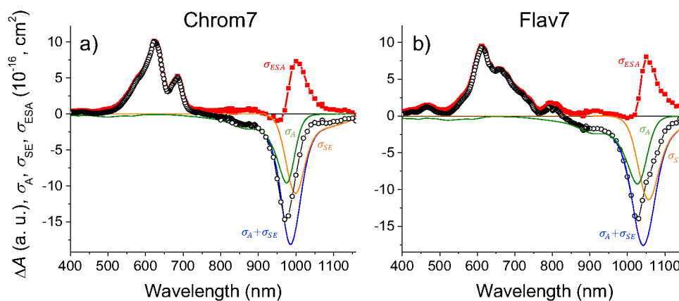
Fig. 10. Chrom7 excited at 990 nm, a), and Flav7 excited at 1042 nm, b), for which the 50-ps \Delta A spectrum from Fig. 2 is scaled (open symbols) to the \sigma_A(\lambda) + \sigma_{SE}(\lambda) sum (with the individual \sigma_A(\lambda) and \sigma_{SE}(\lambda) contributions shown); their difference (solid symbols) is equal to the \sigma_{ESA}(\lambda) spectrum of ESA from S_1 . The \sigma_{ESA}(\lambda) spectral shape is found to be constant from \sim 100 \text{ ps} to delay times as short as 500 fs, Fig. S30.
