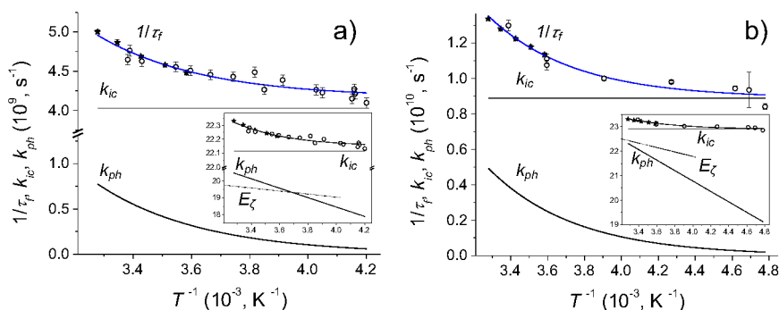
Fig. 8. Chrom7, a), and Flav7, b), in \text{CHCl}_3 : influence of temperature on the inverse S_1 -state lifetime, where \tau_f values were measured by femtosecond transient absorption (open circles) and calculated from the fluorescence quantum yields (solid circles) assuming that k_{rad} is the same as in \text{CH}_2\text{Cl}_2 , Table 1, and the best fits of the 1/\tau_f data using the Arrhenius k_{ph} and temperature independent k_{ic} and k_{rad} rate constants. The insets show the rate constants and \text{CHCl}_3 viscosity, labelled E_\zeta (for comparison, the \zeta values were scaled by a constant factor), plotted on a natural logarithmic scale vs. 10^3 \cdot T^{-1} .
