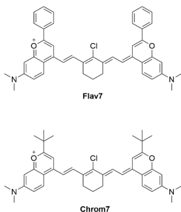
Scheme 1. Structures of the studied dyes (counterion, \text{BF}_4^- ).
