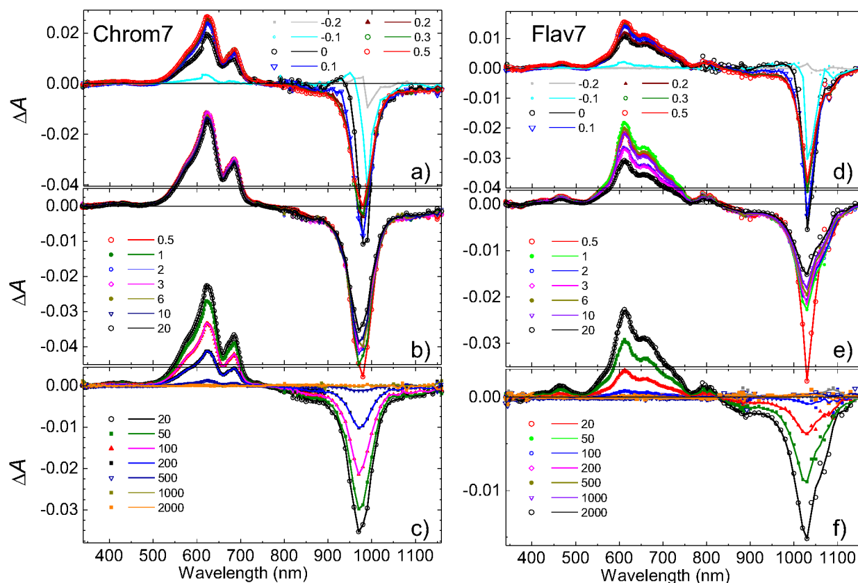
Figure 2. Short- (a, d), intermediate- (b, e), and long- (c, f) time \Delta A spectra of 990-nm excited Chrom7 (a-c) and 1042-nm excited Flav7 (d-e): delay times between excitation and probe pulses expressed in picoseconds are given inside each panel.
