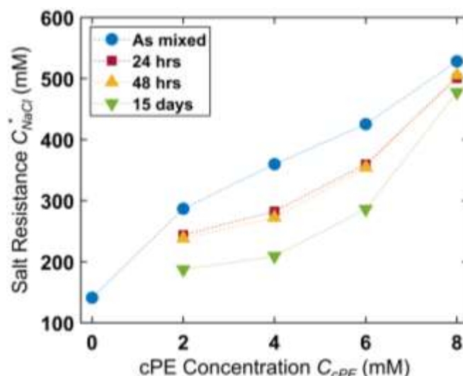
Figure 6: The temporal evolution of the salt resistance C_{NaCl}^* for complex coacervate dispersions. C_{NaCl}^* , corresponding to the maximum salt concentration at which dispersions retained turbidity of 4 \text{ cm}^{-1} irrespective of the PE concentration, is shown as a function of comb polyelectrolyte concentration. C_{NaCl}^* of the complex coacervate dispersions increases with increasing cPE concentration and is maintained for up to 15 days.
