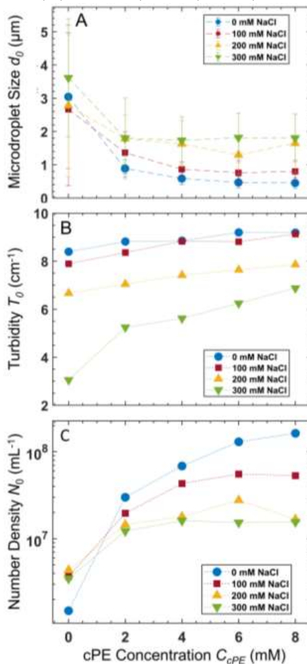
Figure 3: Complex coacervate microdroplet size and number density can be tuned by comb-polyelectrolyte concentration. (A) The initial average microdroplet size decreases with C_{cPE} and increases with C_{salt} . (B) In contrast, the initial turbidity of the dispersion (measured at 400 nm) increases with C_{cPE} and decreases with C_{salt} . (C) The microdroplet number density, estimated from the microdroplet size and dispersion turbidity, mimics turbidity trends.
