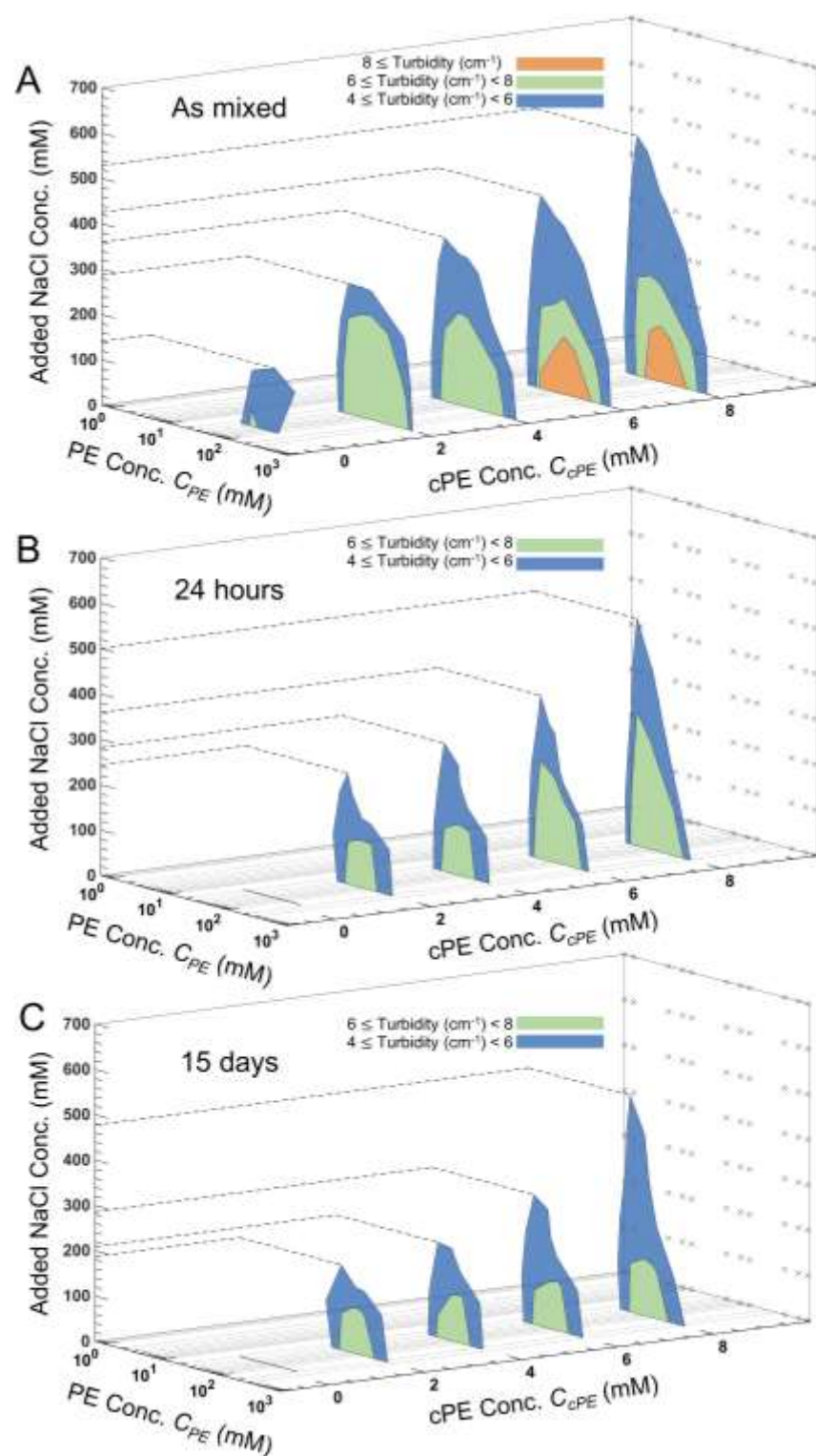
Figure 5: Comb polyelectrolytes stabilize complex coacervate dispersions up to higher salt concentrations, expanding the window of turbidity. (A - C) Turbidity windows are shown over a range of polyelectrolyte (PE, 1:1 charge ratio) and salt concentrations at different comb polyelectrolyte (cPE) concentrations. Increasing cPE concentration is noted to expand the turbidity window, indicating the presence of stabilized microdroplets at higher salt concentrations. (A) shows the turbidity of the as mixed dispersions; (B) and (C) show turbidity windows of these dispersions after 24 hours and 15 days, respectively. The dotted lines denote the salt resistance of the dispersions corresponding to a constant C_{cPE} . The cross symbols on the back panel denote the C_{cPE} - C_{NaCl} compositions where dispersion turbidity was measured.
