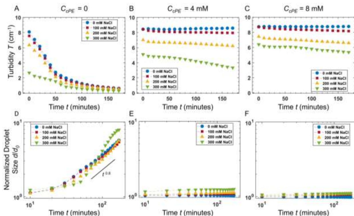
Figure 4: Comb polyelectrolytes improve the stability of complex coacervate dispersions even in the presence of salt. The temporal evolution of (A - C) dispersion turbidity evaluated using a 500 nm incident light and (D - F) the normalized microdroplet size d/d_0 are shown for different salt and cPE concentrations. The rate of coarsening is significantly reduced by increasing cPE concentration, and stable droplets can be obtained even at salt concentrations up to 300 mM.
