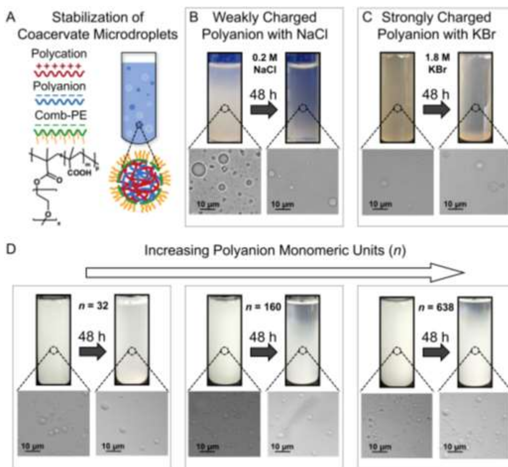
Figure 1: Comb polyelectrolytes (cPEs) stabilize complex coacervate microdroplets. (A) Mixing of oppositely charged polyelectrolytes (1:1 charge ratio) in the presence of cPEs stabilizes the complex coacervate microdroplets against coalescence, resulting in turbid dispersions. r refers to the random copolymer cPEs comprising methacrylic acid and PEG methacrylate. The average values of m , x , and p for the cPEs used in this study are 3.7, 68, and 12.1, respectively. (B) Complex coacervate microdroplets formed with PDADMA (degree of polymerization n = 53 ) and PAA ( n = 54 ), a weak polyelectrolyte, with 0.2 M NaCl were stabilized by anionic cPE. Here, C_{PE} = 62.2 mM and C_{cPE} = 4.8 mM. (C) Droplets formed with PDADMA ( n = 53 ) and PSS ( n = 340 ), a strong polyelectrolyte, with 1.8 M KBr were also stabilized by anionic cPE. Here, C_{PE} = 116.4 mM and C_{cPE} = 50 mM. (D) Coacervate microdroplets with PDADMA ( n = 53 ) and PAA (varying n ) were stabilized by cPE, indicating that cPEs can stabilize complexes with asymmetric linear PEs. In (B - D), dispersion turbidity persisted for 48 hours, and coacervate microdroplets were noted in the corresponding micrographs.
