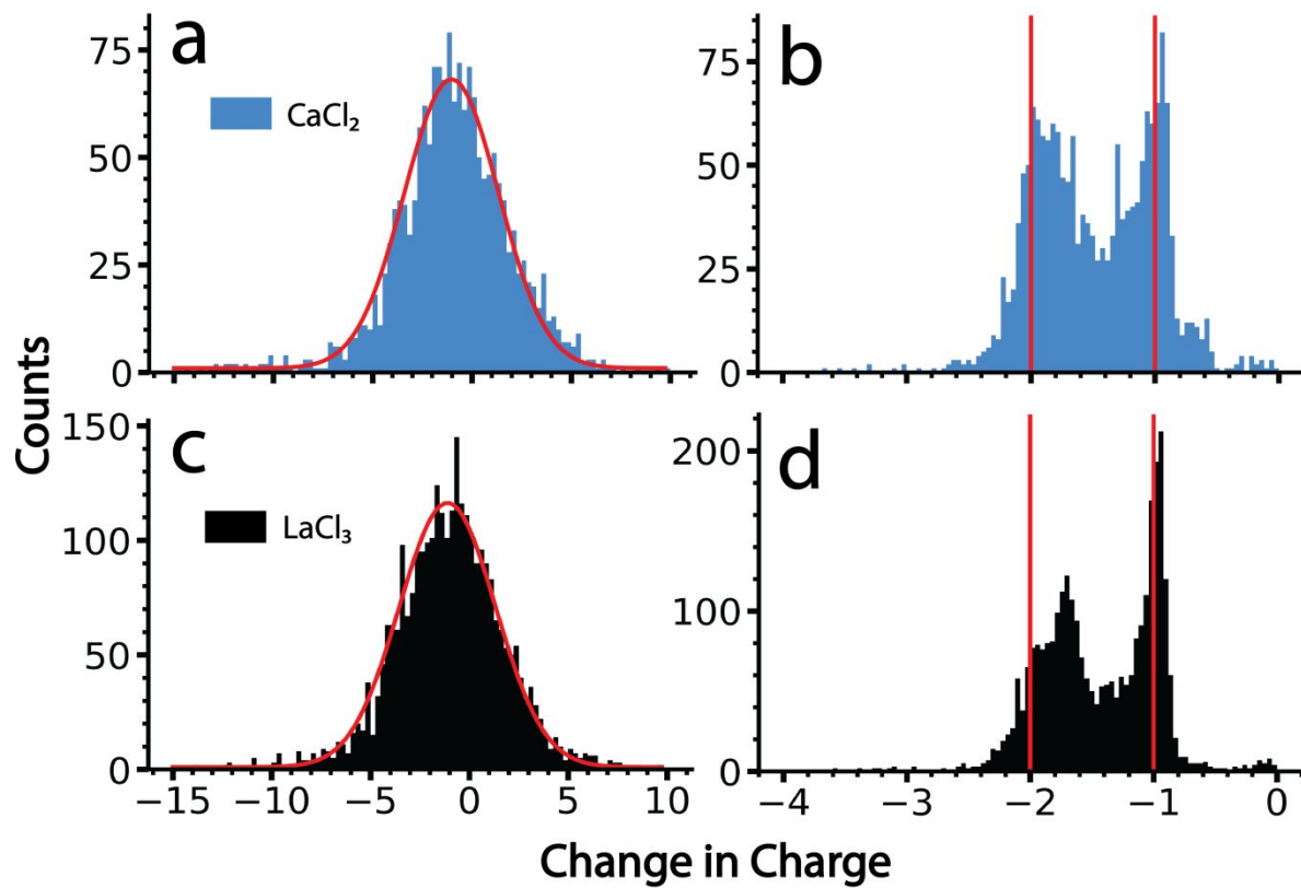
Figure 4. Statistical data showing the change in the charge state of a cluster ion as a result of ion emission events from \text{CaCl}_2 ( a, b ) and \text{LaCl}_3 clusters ( c, d ) determined from the amplitude-based method ( a, c ) and from the frequency-based method ( b, d ). The red lines in ( a ) and ( c ) are Gaussian fits to these data with centers at -1.04 e and -1.11 e , respectively. The red solid lines in ( b ) and ( d ) are centered at -1 e and -2 e , respectively, and demonstrate that emission of +1 and +2 ions from the precursor clusters can be resolved using the frequency-based method. Data for \text{KCl} is not shown because these clusters did not undergo any observable ion emission events.
