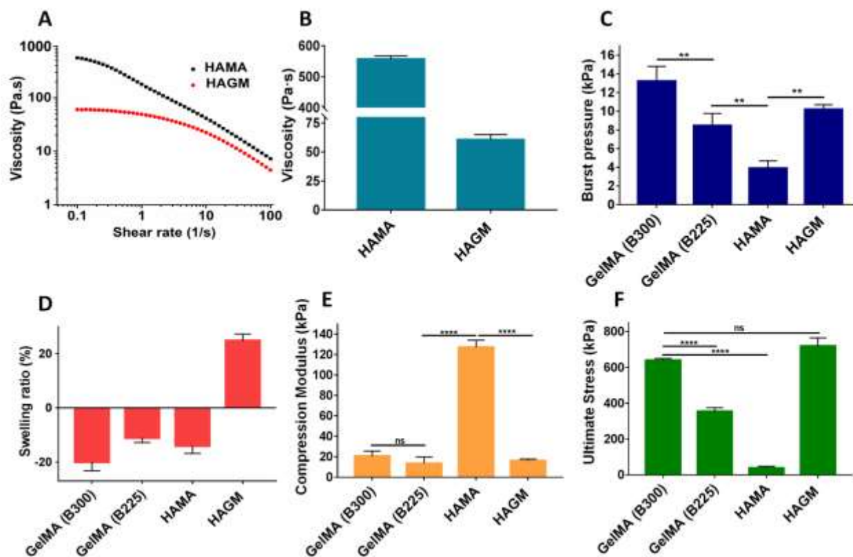
Figure 2. Characterization of prepolymer solution and crosslinked hydrogels formed based on single polymers. (A) Viscosity of HAGM and HAMA as a function of shear rate at 25°C. (B) Viscosity of single polymer-based precursor solutions determined at a shear rate of 0.1 (1/s). (C) Burst pressure of photocrosslinked hydrogels formed based on single polymers. (D) Swelling ratio (%) of photocrosslinked hydrogels formed based on single polymers within the first 24 h upon incubation in DPBS at 37°C. (E) Compression modulus and (F) ultimate strength of photocrosslinked polymers. Data are represented as mean \pm SD (* p <0.05, ** p <0.01, *** p <0.001, **** p <0.0001)
