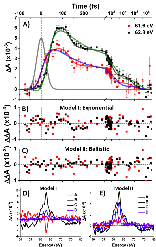
Figure 5. Global analysis of transient M_{2,3} -edge XANES spectroscopy cubane data. A) Data points are shown with error bars ( \pm 1 standard error) and a gaussian profile corresponding to the 48 fs IRF is shown in gray. Fits to the data are shown in solid lines: Model I (exponential) in green and blue, Model II (ballistic) in black and red. Residuals in each model are shown in B) and C) with the same x-axis. Component spectra are shown in D) and E).
