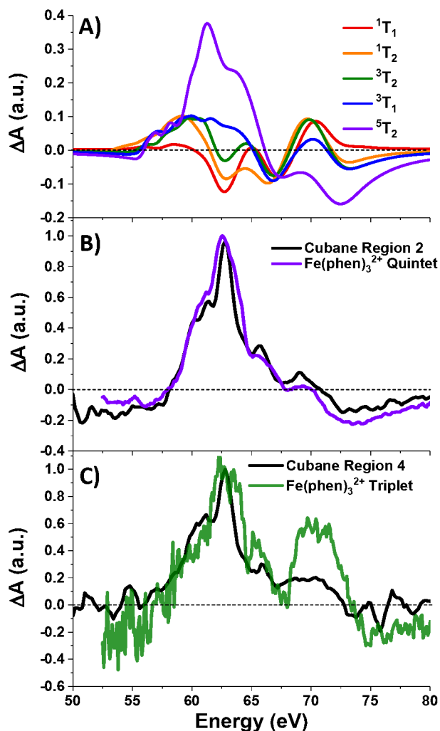
Figure 4. (A) LFM simulations of cubane excited states, and (B) normalized quintet difference spectra of \text{Fe}(\text{phen})_3^{2+} (from ref. 22) compared with that of cubane Region 2, and (C) triplet intermediate spectrum (ibid.) compared with cubane Region 4. \text{Fe}(\text{phen})_3^{2+} spectra have been blue-shifted 5.5 eV.
