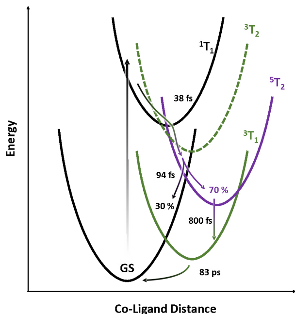
Figure 6. Schematic representing potential energy surfaces in the proposed model.
