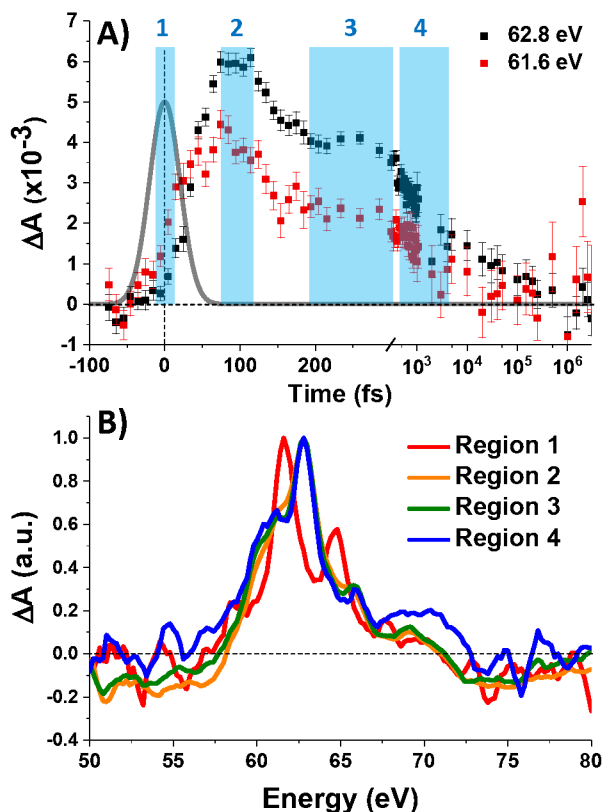
Figure 3. (A) Time traces (data points). Error bars are \pm the standard error. Data traces are integrated \pm 0.2 eV from the listed value. Four integration regions (light blue) are defined. The 48 fs instrument response function is plotted in grey. (B) Normalized and smoothed (5-point [1.0 eV] Savitzky-Golay) time-averaged regions.
