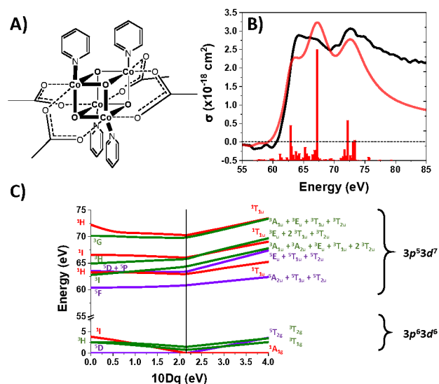
Figure 1. (A) Structure of Co 4 O 4 . (B) Ground state M-edge XANES spectrum. The ligand field multiplet (LFM) simulation and sticks are shown in red. (C) Correlation diagram showing transitions between the 3p^5 3d^6 ground state and 3p^5 3d^7 core-hole excited state as a function of ligand-field strength 10Dq .
