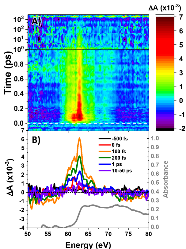
Figure 2. (A) Contour plot of time-resolved M-edge XANES spectra. Time zero is indicated in the dashed white line. (B) Selected spectral slices with the ground state Co_4O_4 spectrum in grey for comparison. The data are binned to 0.2 eV intervals.
