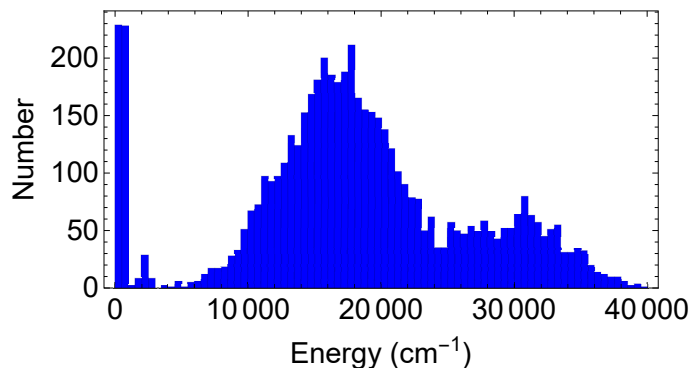
Fig. 2 Histogram of energies for geometries used as the dataset for acetyl-acetone. The bin size for the abscissa is 500 \text{ cm}^{-1} . The database has 5,500 energies and (not shown) 45 \times 5,500 gradient components.
